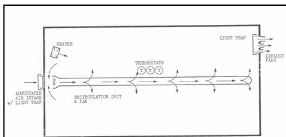
FIGURE 2: VENTILATION SYSTEM FOR OVERWINTERING HIVES
